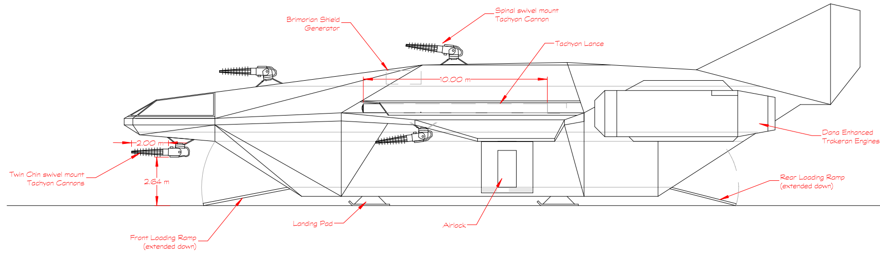
Side Elevation
