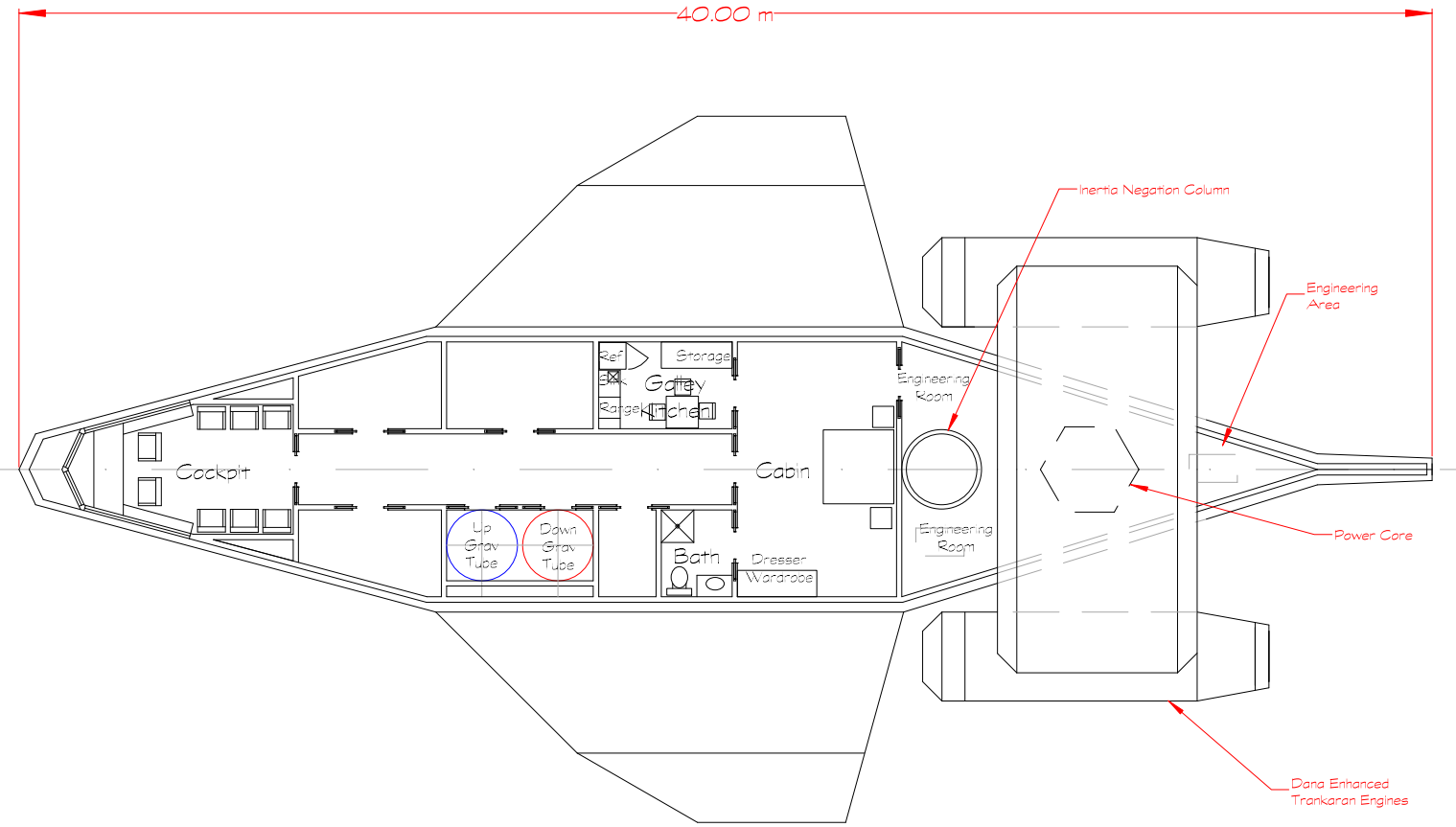
Cockpit Level Floor Plan
